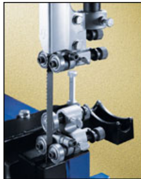
Upper and Lower Ball Bearing Blade Guide System.
