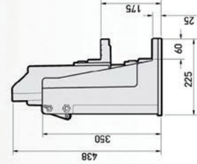
Position 1: Extremely low pick up point.
